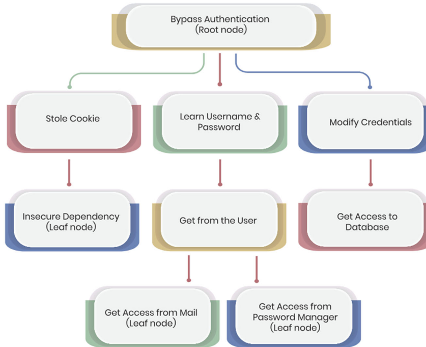
Figure 1: Example Attack Tree from the British National Cyber Centre
