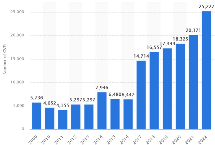
Figure 1: CVE (Common Vulnerability and Exposures) counts from 2009 – 2022
