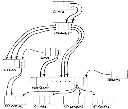
Figure 1: The data structures of HijackGL's declarative representation of geometry. This figure does not show the complete set of information tracked by HijackGL. Rather, it is meant to indicate the overall structure.
