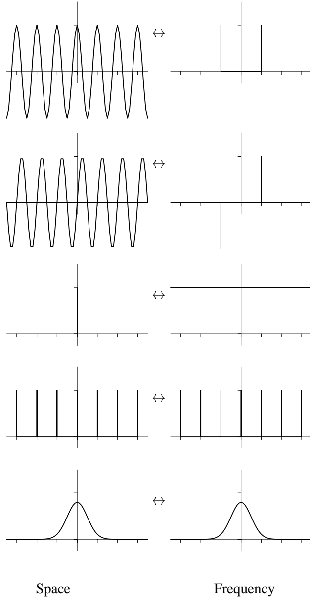
Figure 5: Fourier transform pairs. From top to bottom: \cos \omega x , \sin \omega x , \delta(x) , \text{shah}(x) , and e^{-x^2} .
