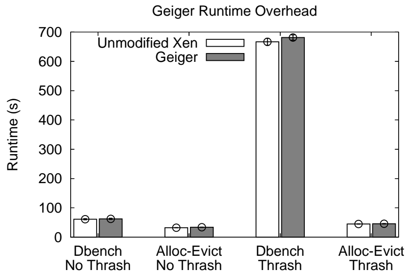
Figure 5.8 Geiger Runtime Overhead. The figure shows that Geiger imposes very small runtime overheads for two workloads that stress its inference heuristics.
