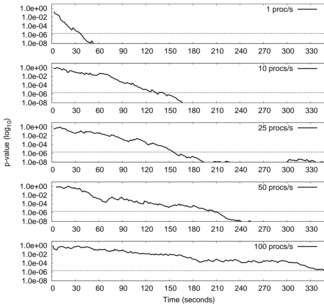
Figure 6.3 Detection Timelines. The figure shows a timeline of the hypothesis test p-values used in the detection process for each of several levels of process creation/exit activity. The p-values approach the detection threshold over time.
