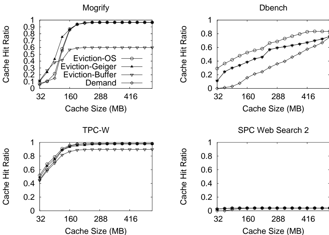
Figure 5.13 Secondary Cache Hit Ratio. The figure compares the cache hit ratio in a secondary storage cache for various workloads when demand placement ( Demand ), eviction placement based on inferred evictions ( Eviction-Buffer and Eviction-Geiger ), and eviction placement based on actual evictions ( Eviction-OS ) is used. Experiments are performed using cache sizes from 32 MB to 512 MB.
