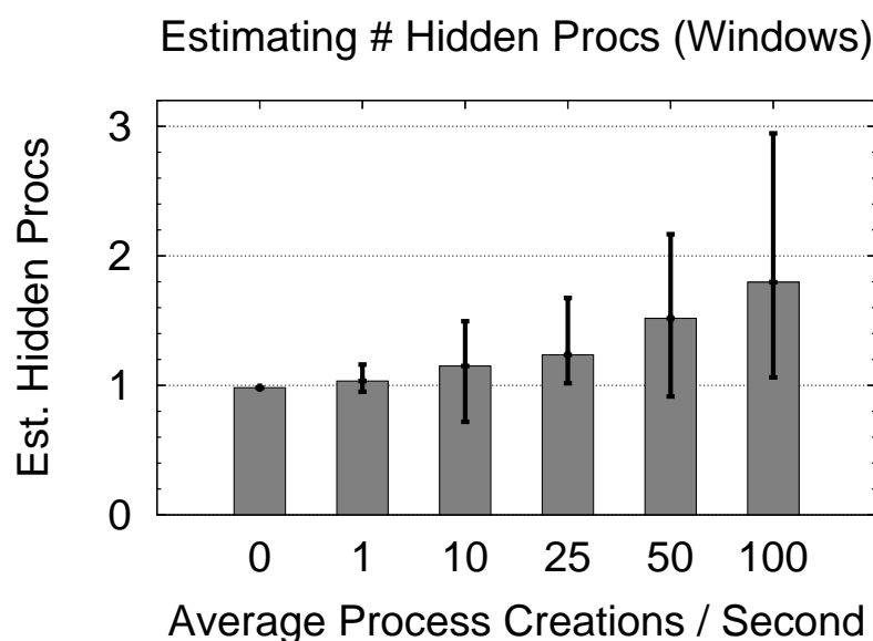
Figure 6.5 Estimating the Number of Hidden Process. The figure shows how the estimate of the number of hidden processes obtained from the detection phase varies for Windows as process creation and exit activity increases from 0 processes/second to 100 processes/second when a single process has been hidden. The values shown are an average of 10 trials. Error bars show the minimum and maximum hidden process estimate observed.
