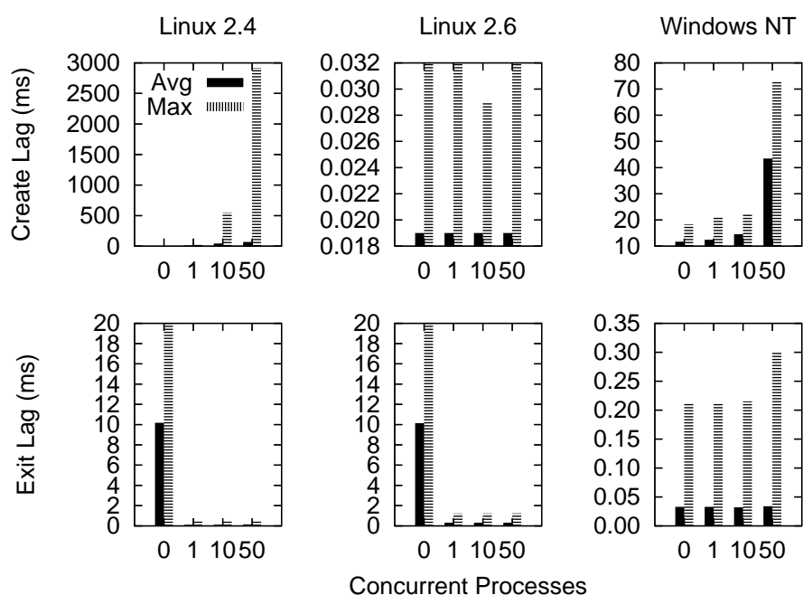
Figure 4.2 Lag vs. System Load. The figure shows average and maximum create and exit lag time measurements for a variety of system load levels in each of our x86 evaluation environments. Average and worst case create lag are affected by system load in Linux 2.4 and Windows, but are small and nearly constant under Linux 2.6. Except for a large exit lag with no competing processes on Linux, exit lag does not appear to be sensitive to system load.
