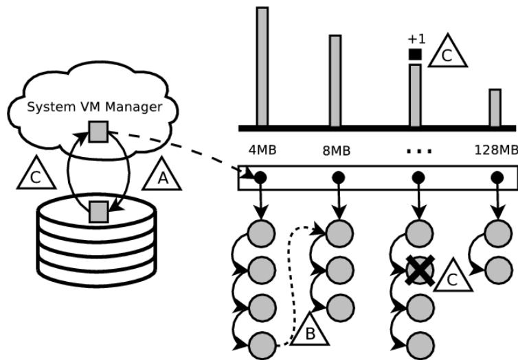
Figure 5.9 MemRx Operation. The figure shows a schematic of the cache simulation implemented by MemRx. A) When a page is evicted by a guest, this event is detected by MemRx and an entry is added to the head of a series of queues. B) If necessary, queue entries ripple from the tail of one queue to the head of the next. C) Upon reload, the associated queue entry is removed and an array entry associated with that queue is incremented. Each entry tracks which sub-queue it appears in to enable fast depth estimation.
