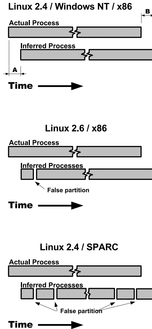
Figure 4.1 Effects of error. The figure shows where each type of process identification error occurs for each tested platform. Error is either lag between when the true event occurs and when the VMM detects it, (e.g., A and B in the figure) or consists of falsely partitioning a single OS process into multiple inferred processes. In Linux 2.6/x86, this only occurs on exec , which typically happens immediately after fork . On SPARC this partitioning happens whenever a process calls either fork or exec .
