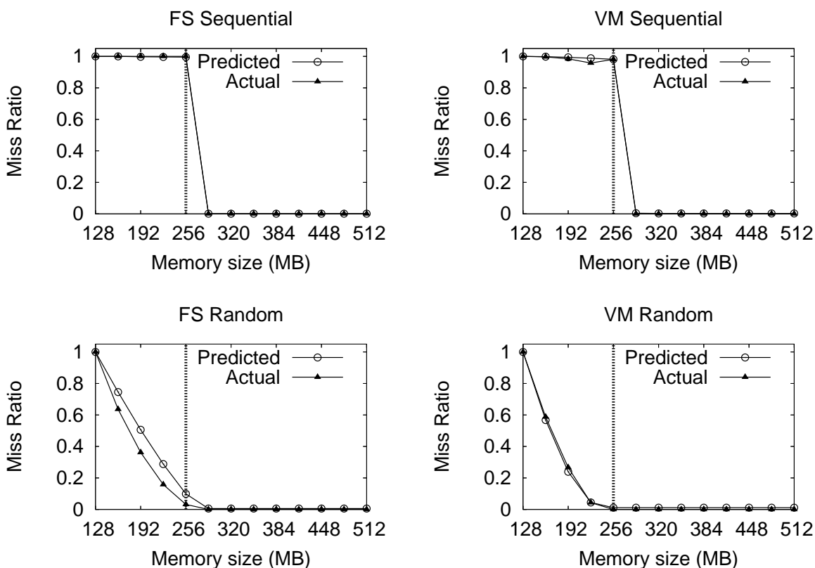
Figure 5.11 VMM-MemRx Predicted vs. Actual Miss Ratio. The figure shows the miss ratio predicted by VMM-MemRx vs. the actual miss ratio measured for varying memory sizes. The known working set of 256 MB is marked by a vertical dashed line.
