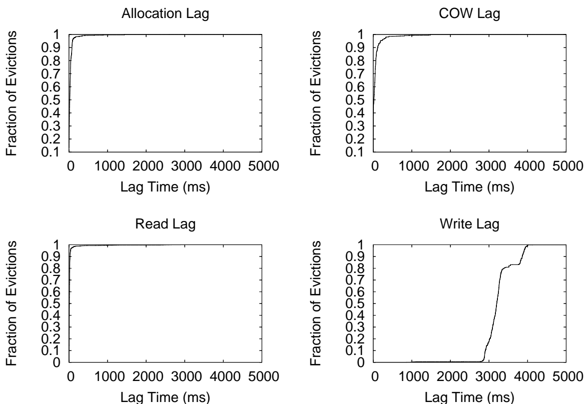
Figure 5.4 Eviction Lag. The figure shows the cumulative lag distribution for microbenchmarks that isolate each eviction type.
