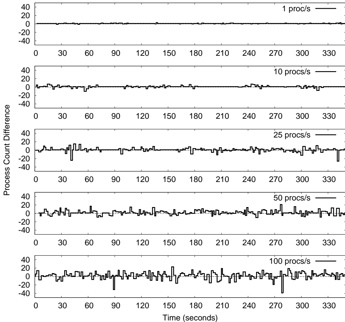
Figure 6.2 Process Count Difference Timelines. The figure shows a timeline of the difference between the process list length obtained within the VMM and from the guest operating system for various levels of process creation and exit activity. As process activity increases the variability in the measured difference increases.
