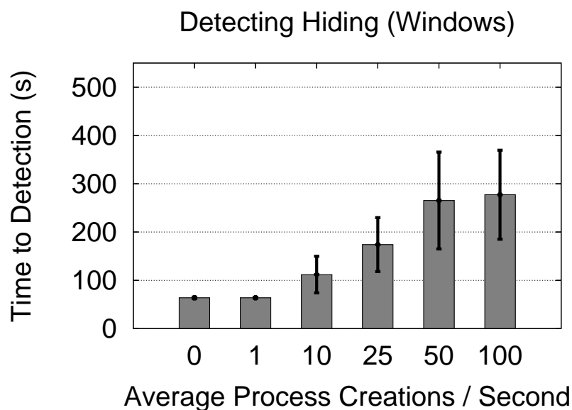
Figure 6.4 Time to Detection. The figure shows how the time to detect a hidden process varies for Windows as process creation and exit activity increases from 0 processes/second to 100 processes/second. The values shown are an average of 10 trials. Error bars show the standard deviation of detection time.
