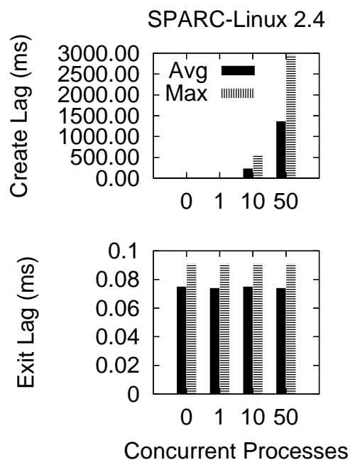
Figure 4.4 Lag vs. System Load, SPARC. The figure shows average and maximum create and exit lag time measurements for the same experiments described in Figure 4.2. Create lag grows with system load. Exit lag is small and nearly constant, independent of load.
