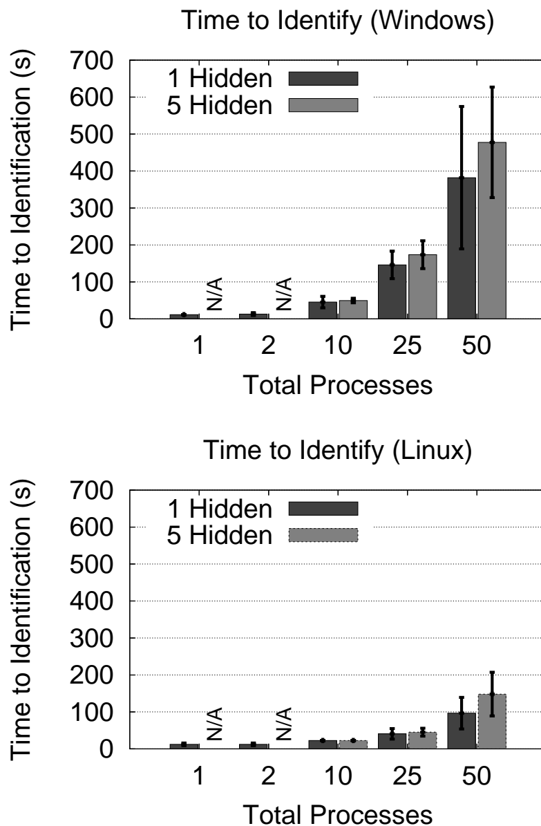
Figure 6.9 Time to Identification. The figure shows how the time to identify hidden processes grows as the number of total active processes increases from 1 to 50 processes for both Windows (upper graph) and Linux (lower graph). The values shown are an average of 10 trials. Lycosid identified the correct hidden processes in all cases on both platforms. Error bars show the standard deviation of identification time. The left bar corresponds to trials in which a single process was hidden. The right bar shows results when 5 processes were hidden.
