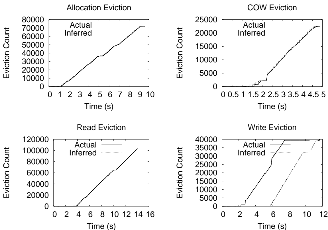
Figure 5.3 Eviction Inference Counts. The figure compares inferred vs. actual eviction counts over time for microbenchmarks that isolate each eviction type inferred by Geiger.
