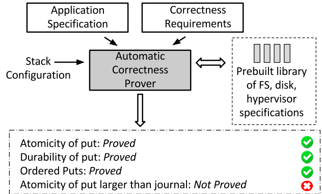
Figure 1: System Architecture. The figure shows a typical workflow – the application specification, correctness requirements, and storage stack configuration are obtained as input, appropriate specifications from the prebuilt library are selected, and finally, the required guarantees are proved/disproved.
