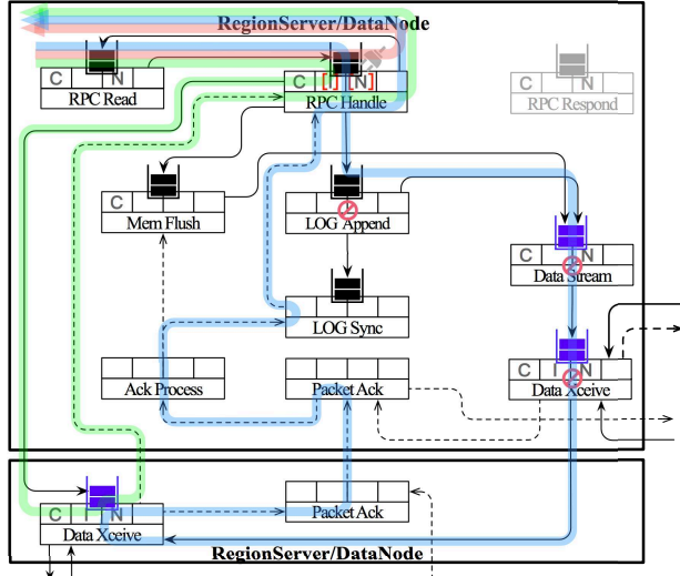
Figure 16: Muzzled-HBase TAD.
