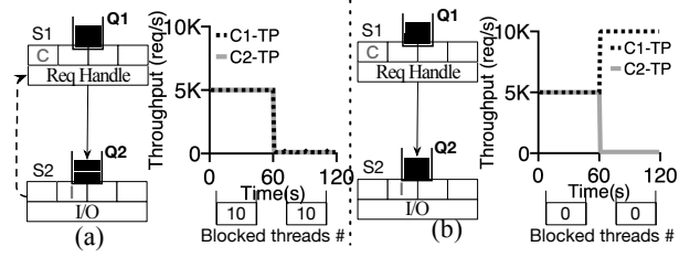
Figure 11: The Blocking Problem. Initially both C1 and C2 issue requests that require 100 \mu s CPU time and can be completed within the Req Handle Stage. At time 60, C2 switches to an I/O intensive workload where each request additionally requires 100 KB I/O at the I/O stage. C1 continues to issue CPU-only requests. The table below shows the average number of blocking threads in Req Handle (10 threads in total).
