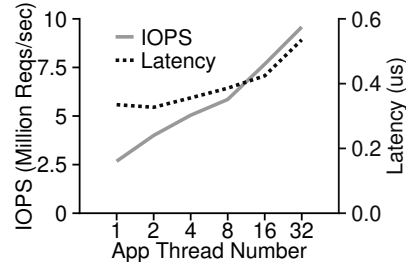
Figure 3: Performance of Communication Channel
