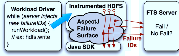
Figure 2: FTS Framework.
