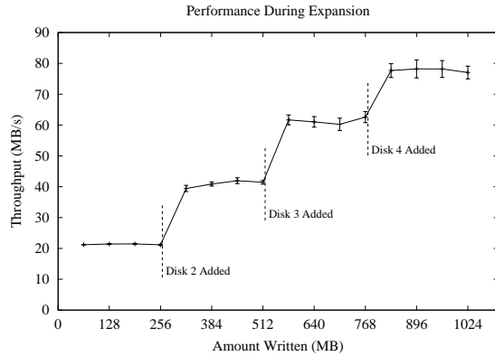
Figure 4: Storage Expansion. The graph plots the performance of I-LFS during storage expansion. The experiment begins with I-LFS writing to a single disk. Each time 256 MB is written, a new disk is brought on-line, and I-LFS immediately begins writing to it for increased performance. Disk expansion is accomplished via a simple command, which adds the disk (or region) to the file system without downtime.
