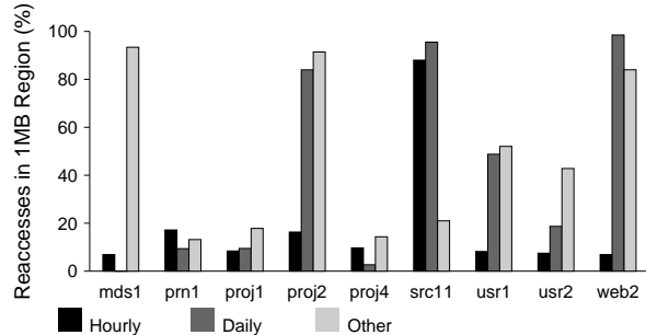
Figure 4: Consecutive Length
