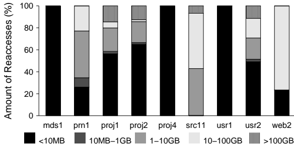
Figure 3: Reuse Distance
