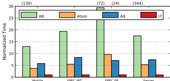
Figure 2. Execution Time Normalized to i7.
