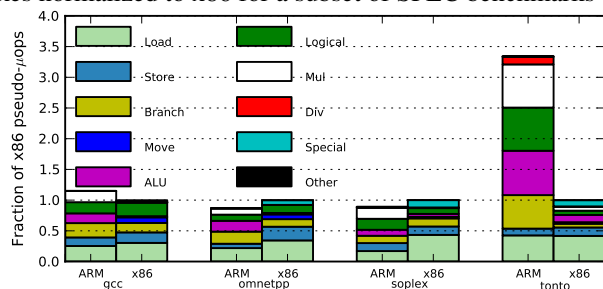
Figure 6. Selected Instruction Counts (Emulated).
