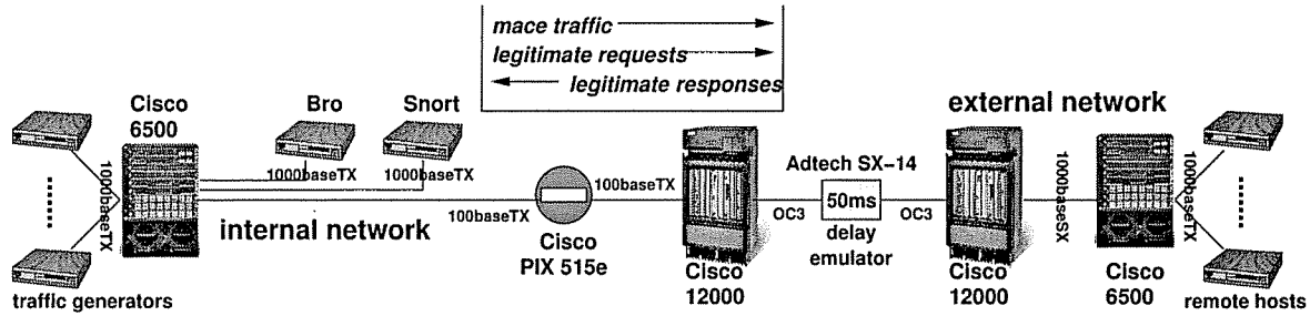
Fig. 3. Experimental Environment. Legitimate and malicious traffic originate from the internal network and are directed toward a host on the external network. The PIX firewall separates the inside and outside networks and performs network address translation.
