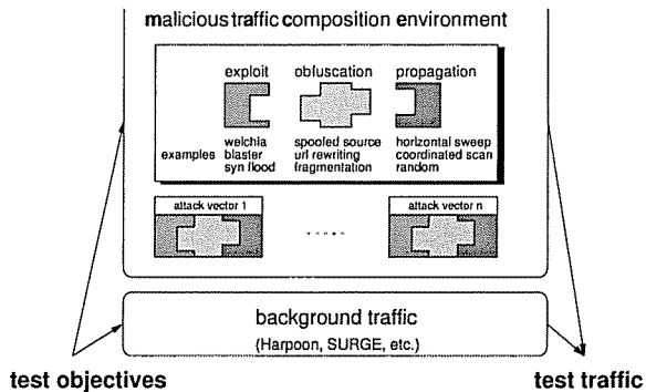
Fig. 1. The MACE architecture. Test objectives inform the selection and composition of exploit, obfuscation, and propagation components into a series of attack vectors. Existing tools such as Harpoon produce the desired benign background traffic.
