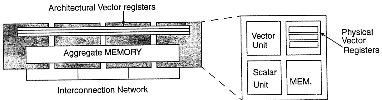
FIGURE 1. DIVA system comprised of four nodes. Each node contains some part of the system memory along with a processor and a vector unit. In this example each node has three physical vector registers. An application running on all four nodes (occupying all their memory) refers to architectural vector registers that are the aggregate of four physical vector register (one of every node).
