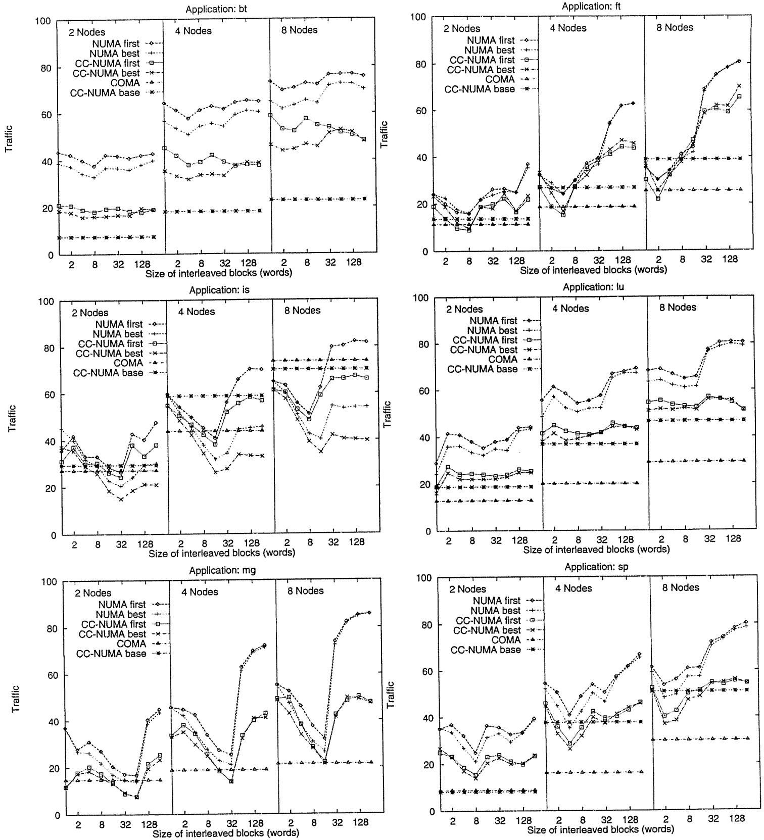
FIGURE 9. Benchmark Traffic
