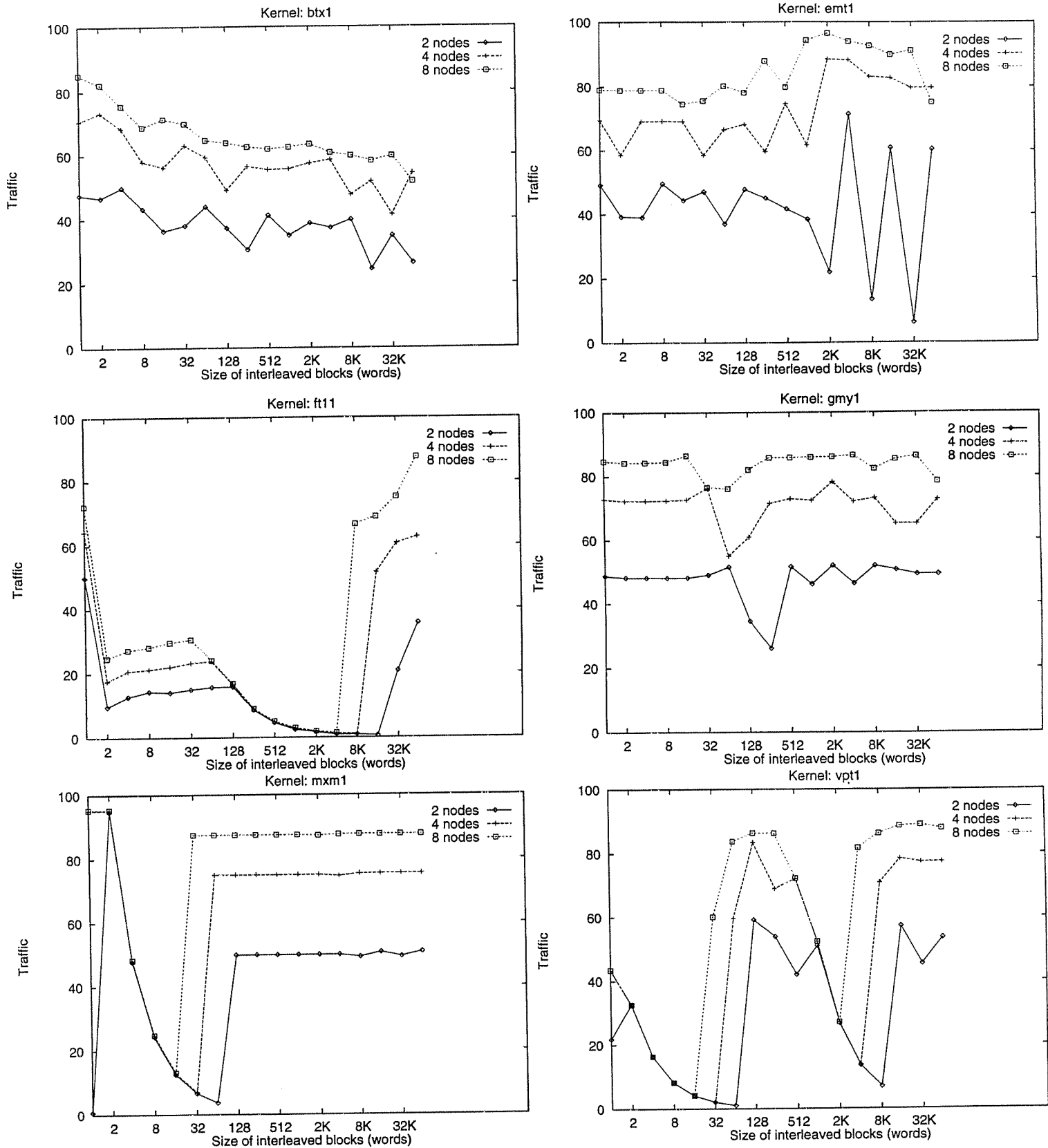
FIGURE 6. Kernel Traffic
