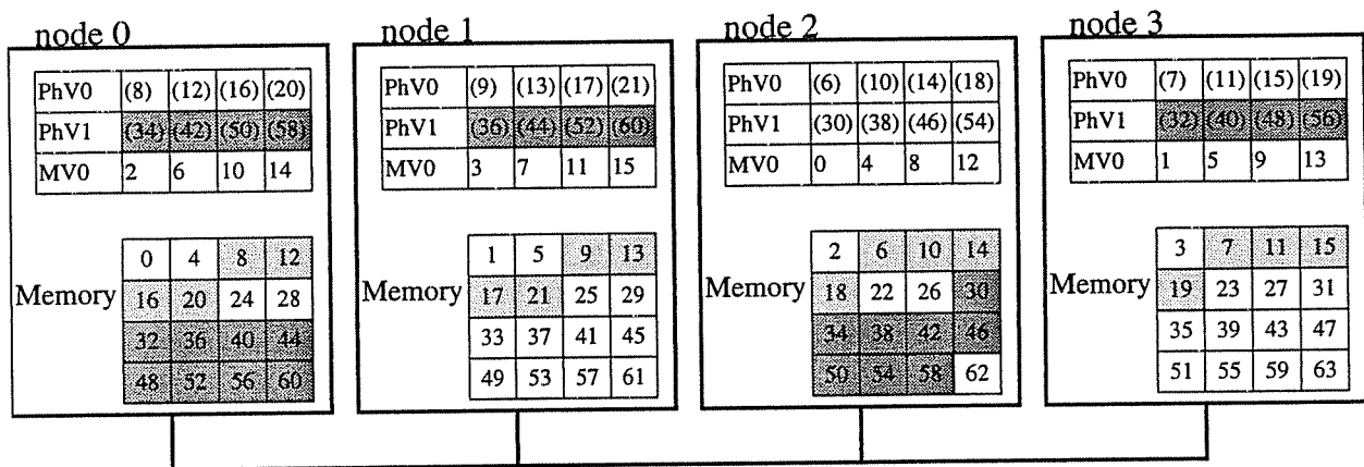
FIGURE 4. State of the DIVA system after executing the two loads of the example code. V0 elements are loaded locally, because mapping vector MV0 is set to mirror vector A in memory. 12 elements of v1, however, require remote communication according to the same mapping vector.
