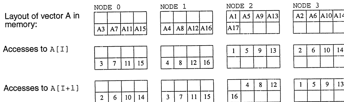
FIGURE 8. Alignment problems when distributing consecutive elements around the nodes (second formula).
