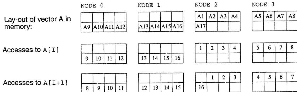
FIGURE 7. Alignment problems when distributing memory vectors in groups of contiguous elements (first formula).
