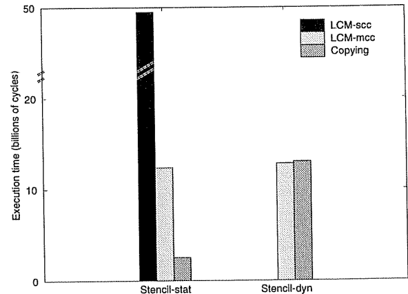
Figure 2: Stencil execution time.
