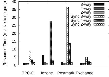
Figure 7: Shared-control ganging
